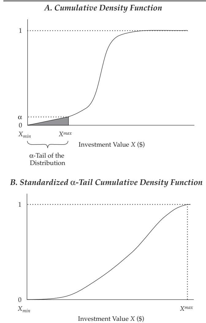
Figure 11. CDF and Standardized \alpha -Tail CDF
